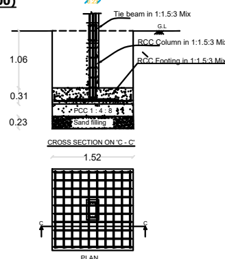
DETAILS OF COLUMNS
