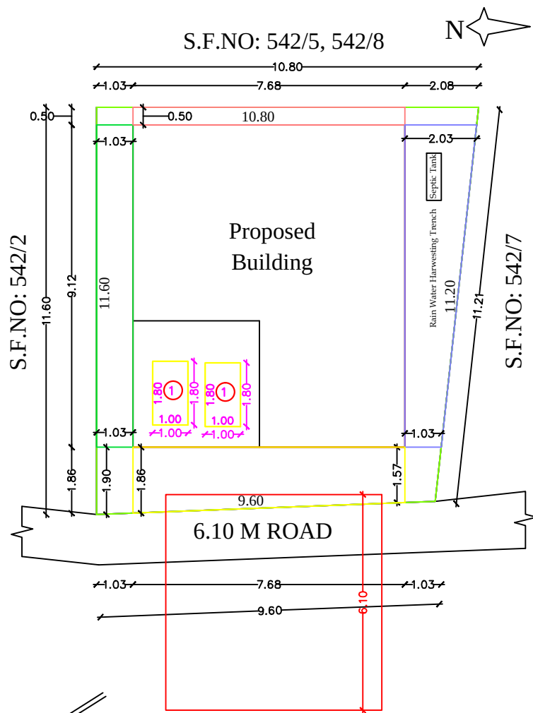
SITE PLAN
