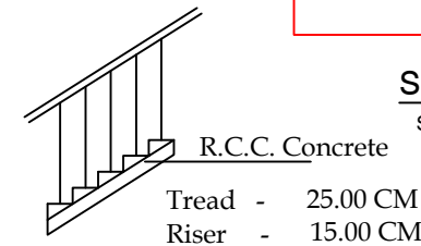
Staircase details
