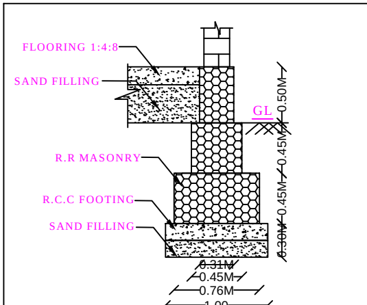
TYPICAL SECTION OF R.R MASONRY FOOTING DETAILS
