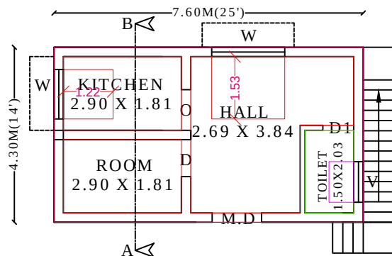
PRO.GROUND FLOOR PLAN (SOUTH FACING)
