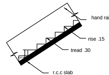
STAIR
