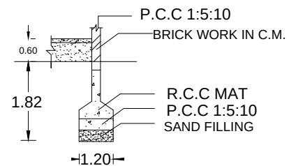
FOUNDATION DETAILS
