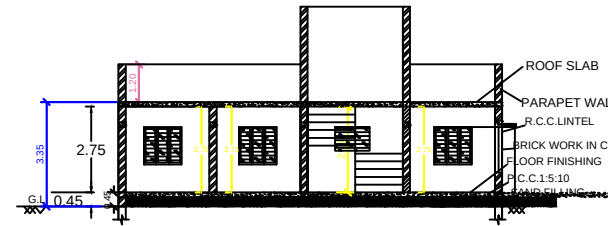
SECTION ON SS
