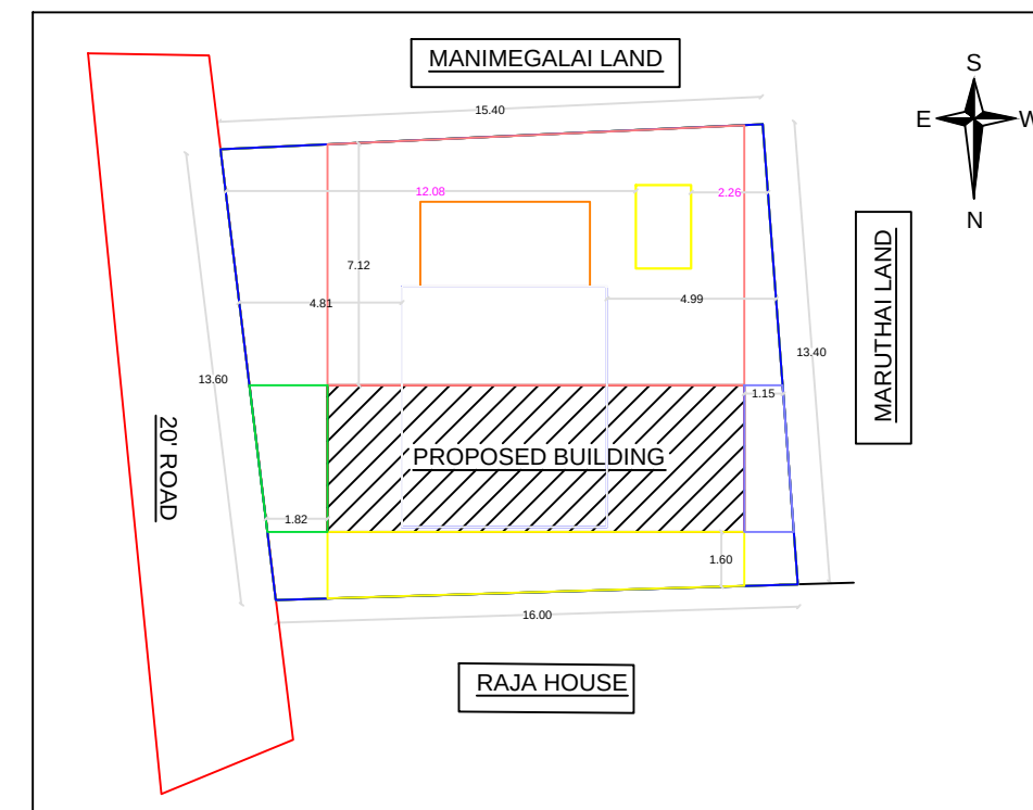
SITE PLAN : [1:100] SCALE
