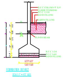
FOUNDATION DETAILS
