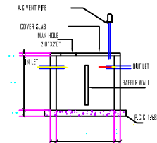
CROSS SECTION OF SEPTIC TANK
