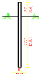
BORE WELL
