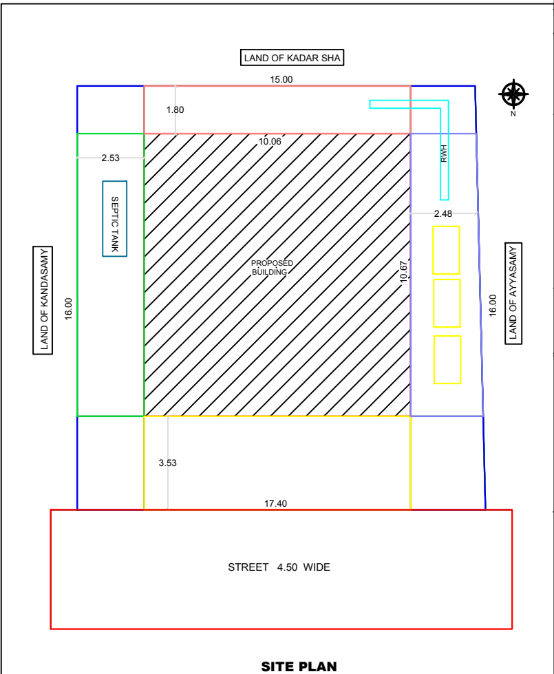
SITE PLAN
