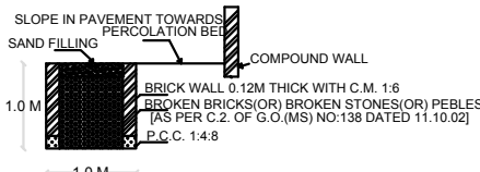
SECTION OF RAIN WATER PERCOLATION BED
