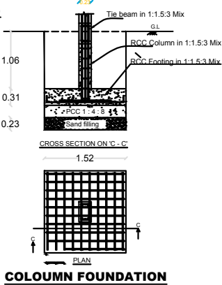
COLOUMN FOUNDATION
