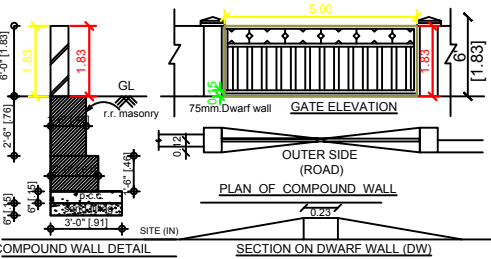
DETAILS OF COMPOUND WALL
