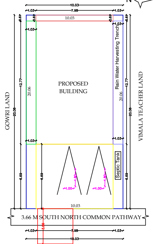
SITE PLAN
