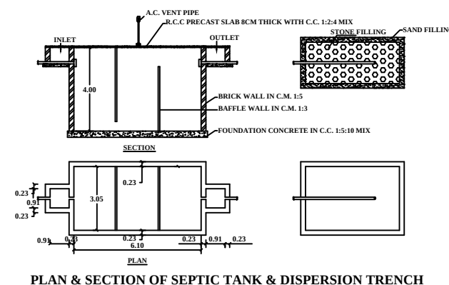
PLAN & SECTION OF SEPTIC TANK & DISPERSION TRENCH
