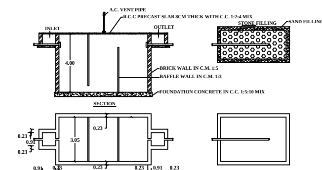
PLAN & SECTION OF SEPTIC TANK & DISPERSION TRENCH
