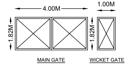
MAIN GATE WICKET GATE
