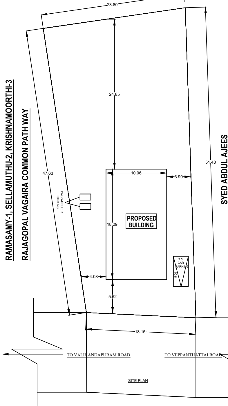
SITE PLAN
