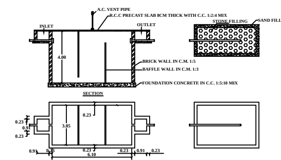
PLAN PLAN & SECTION OF SEPTIC TANK & DISPERSION TRENCH
