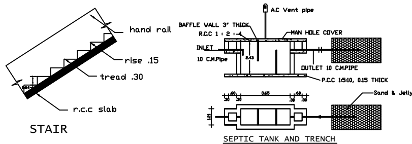
SEPTIC TANK AND TRENCH
