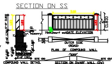
SECTION ON SS
