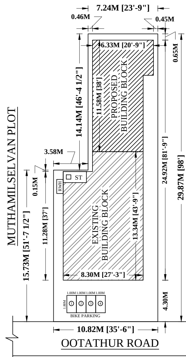
SITE PLAN SCALE IN -1:200
