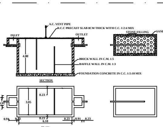
PLAN & SECTION OF SEPTIC TANK & DISPERSION TRENCH
