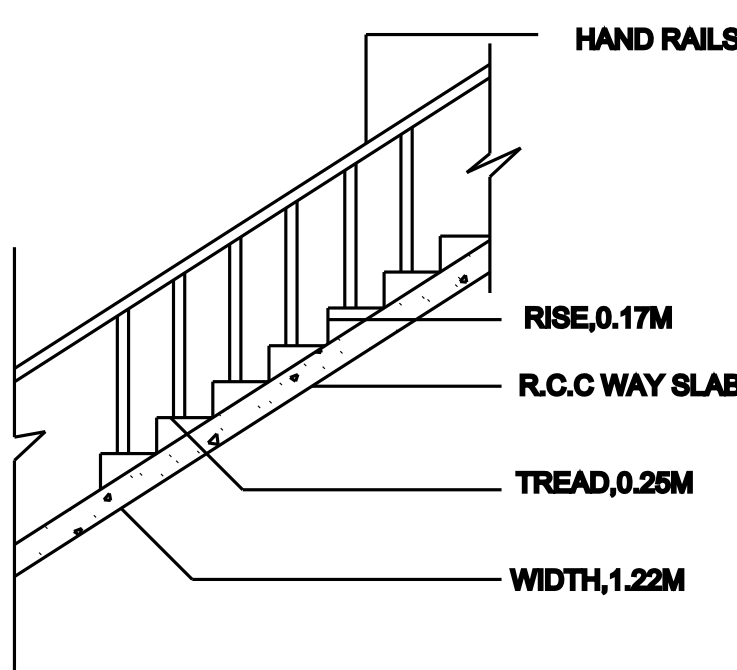
SECTION ON STEP
