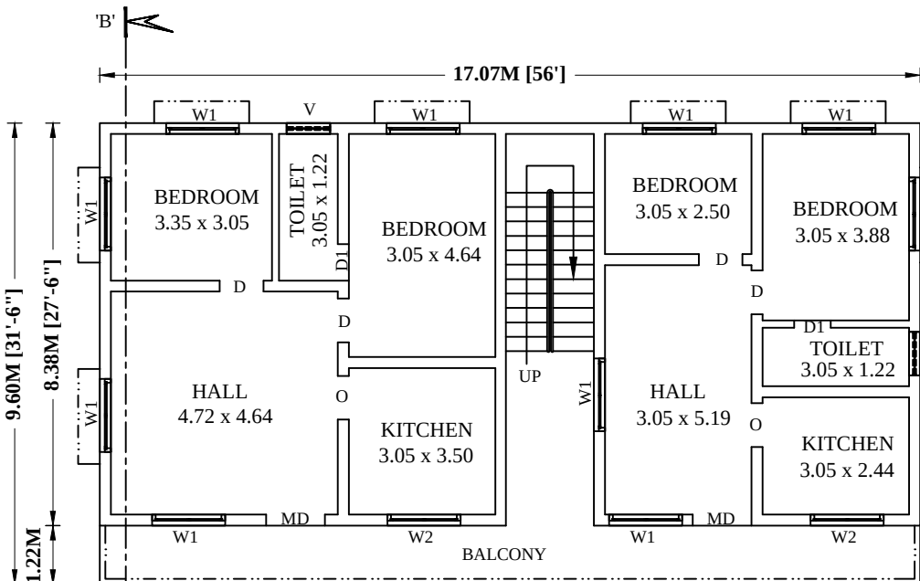
FIRS FLOOR PLAN
