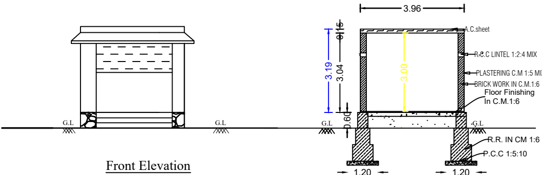
Section On-"AB"
