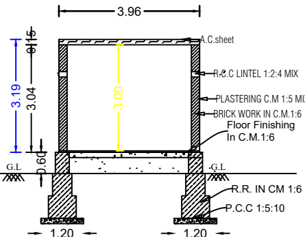
Section On-"AB"
