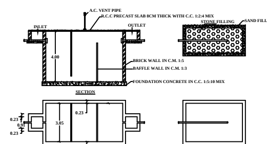
PLAN PLAN & SECTION OF SEPTIC TANK & DISPERSION TRENCH
