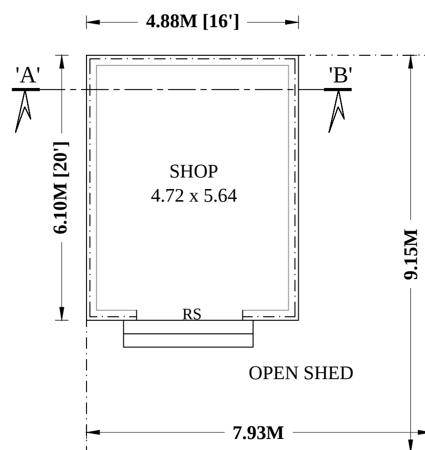
SHOP PLAN
