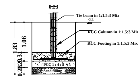
COLOUMN FOUNDATION DETAILS
