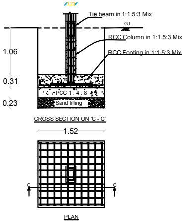
COLOUMN FOUNDATION
