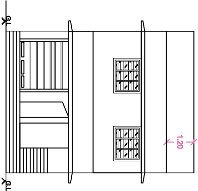
FRONT ELEVATION
