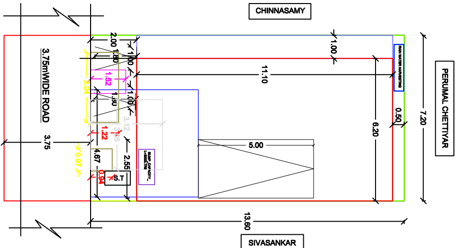
SITE PLAN
