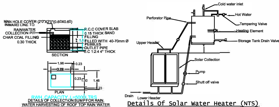
Details Of Solar Water Heater (NTS)
