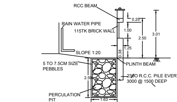
RAINWATER HARVESTING
