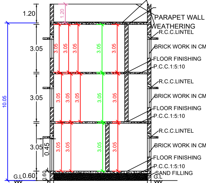
SECTION ON SS
