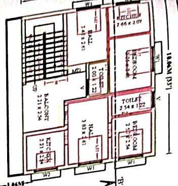
PROPOSED SECOND FLOOR PLAN
