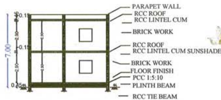
SECTION XX
