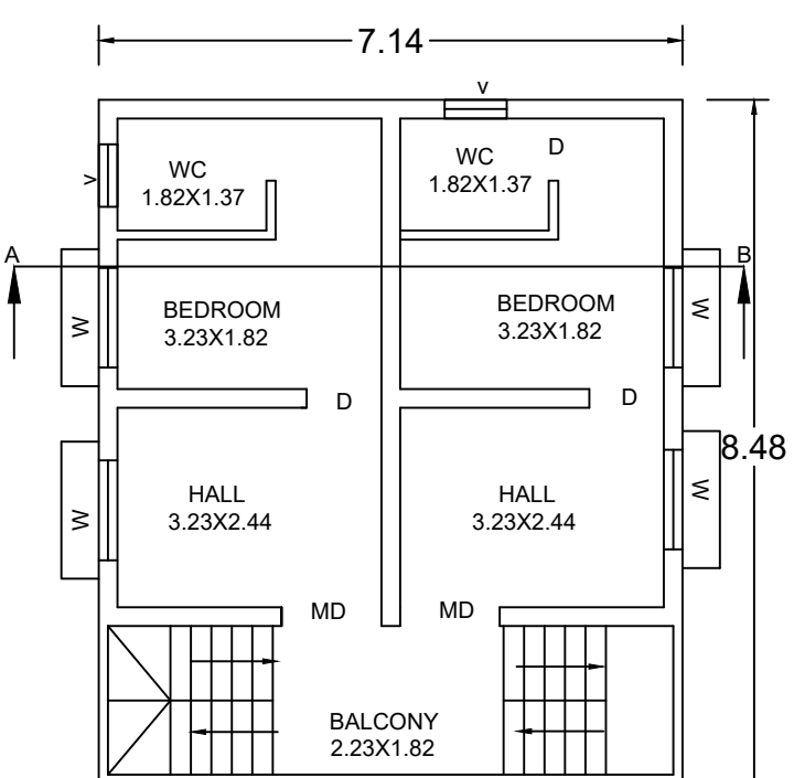
PRO.FIRST FLOOR PLAN
