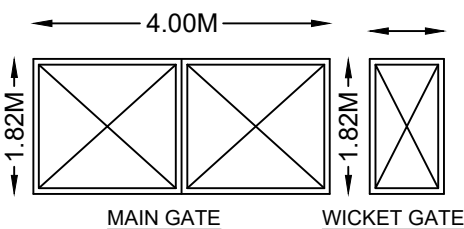
MAIN GATE WICKET GATE
