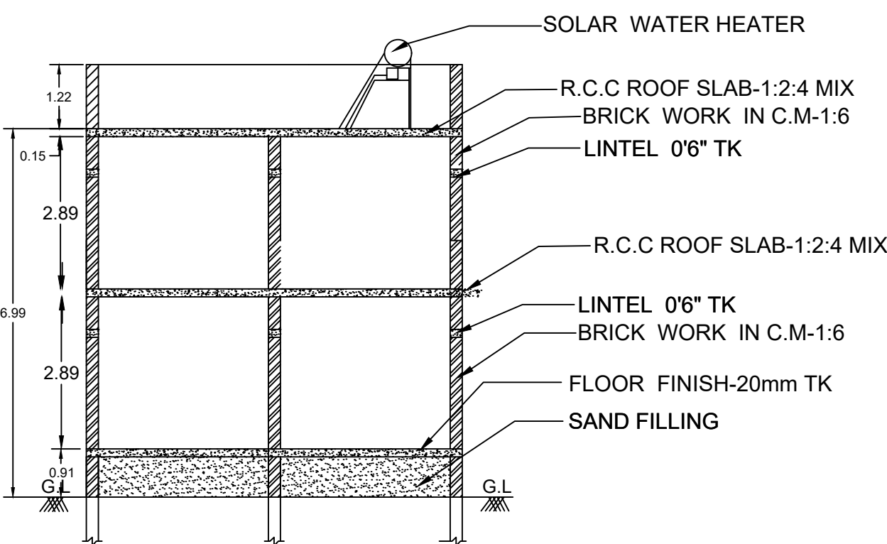
CROSS SECTION (A-B)
