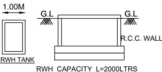
RWH_CAPACITY_L=2000LTRS
