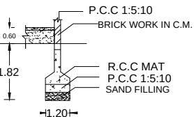
FOUNDATION DETAILS
