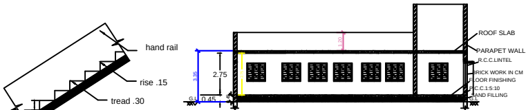
SECTION ON SS
