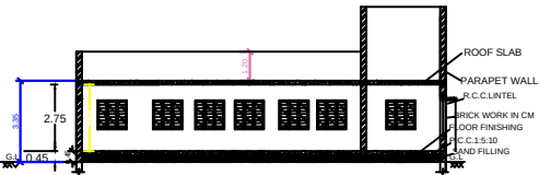
SECTION ON SS
