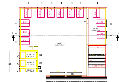
ROUND FLOOR
