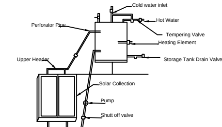
Details Of Solar Water Heater (NTS)
