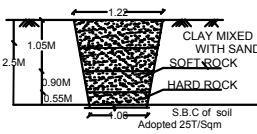
TRIAL PIT DETAILS
