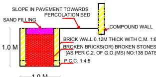
SECTION OF RAIN WATER PERCOLATION BED
