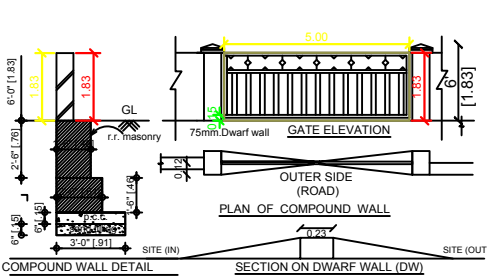
DETAILS OF COMPOUND WALL
