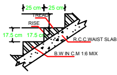
SECTION OF STAIRCASE
