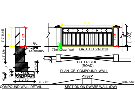
DETAILS OF COMPOUND WALL
