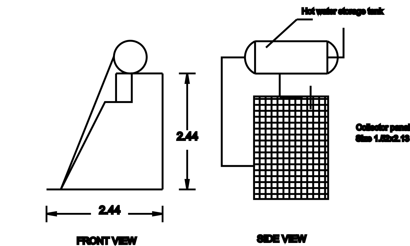
SOLAR WATER HEATER DETAILS [SCALE 1:100]
