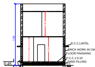
SECTION ON SS
