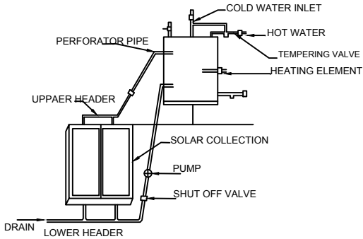
DETAILS OF SOLAR WATER HARVESTING (NTS)
