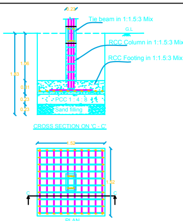
COLOUMN FOUNDATION DETAILS
