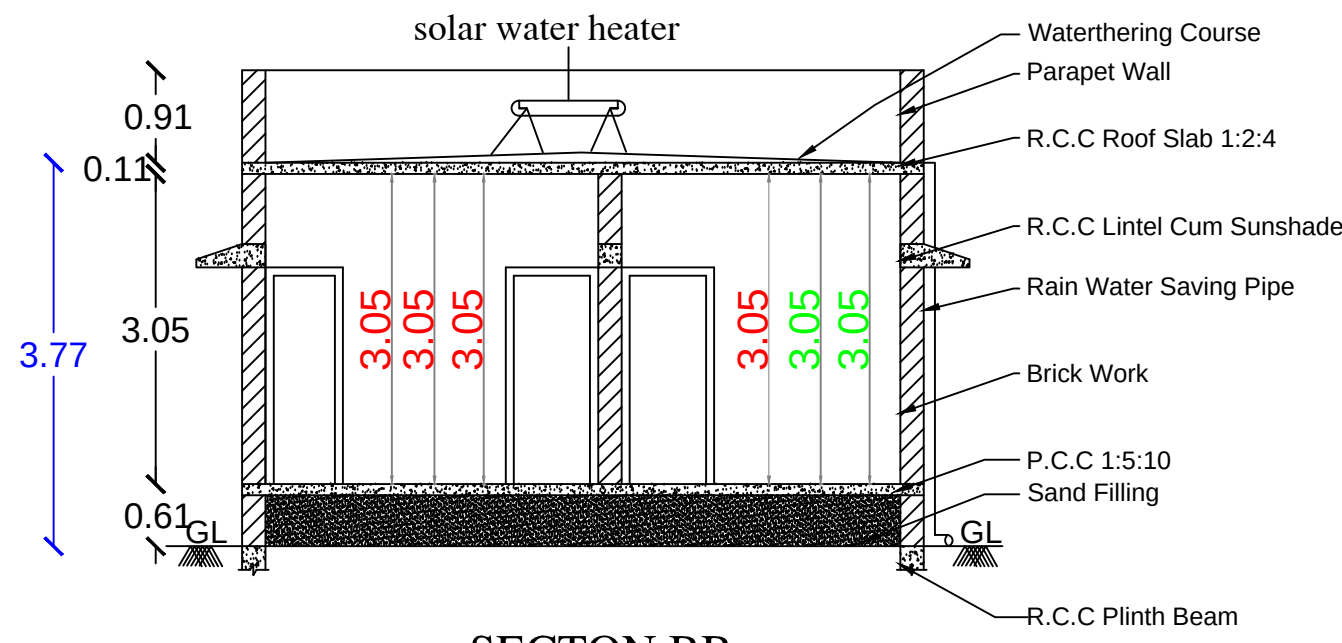
SECTION BB
