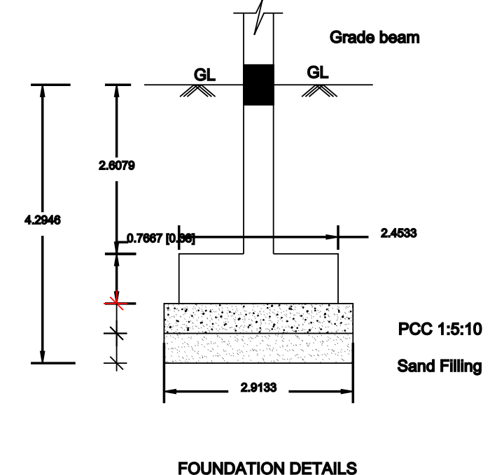
FOUNDATION DETAILS
