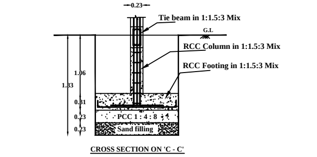
COLOUMN FOUNDATION DETAILS
