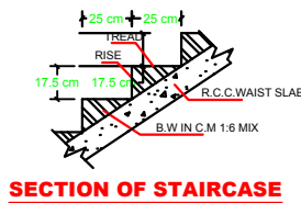
SECTION OF STAIRCASE
