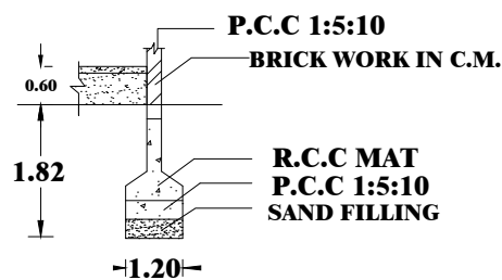
FOUNDATION DETAILS
