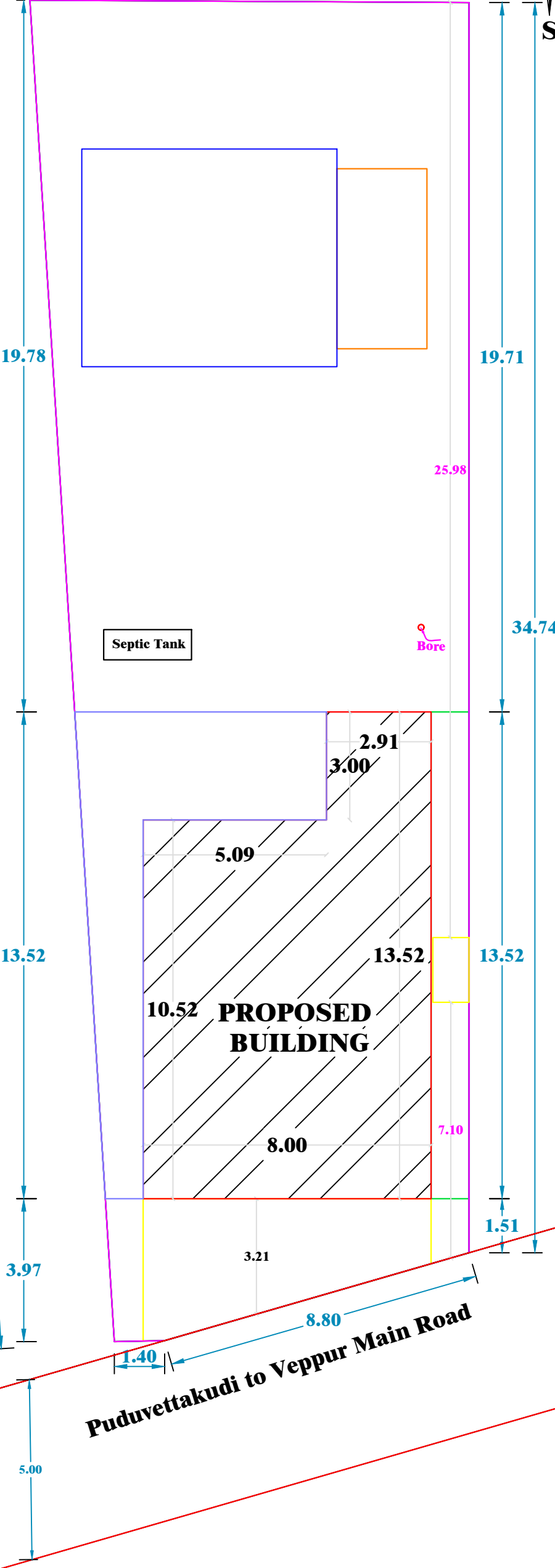
SITE PLAN [1:100] SCALE
