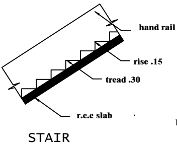
STAIR
