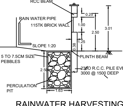
RAINWATER HARVESTING
