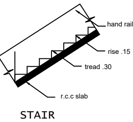
STAIR
