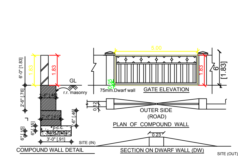
DETAILS OF COMPOUND WALL
