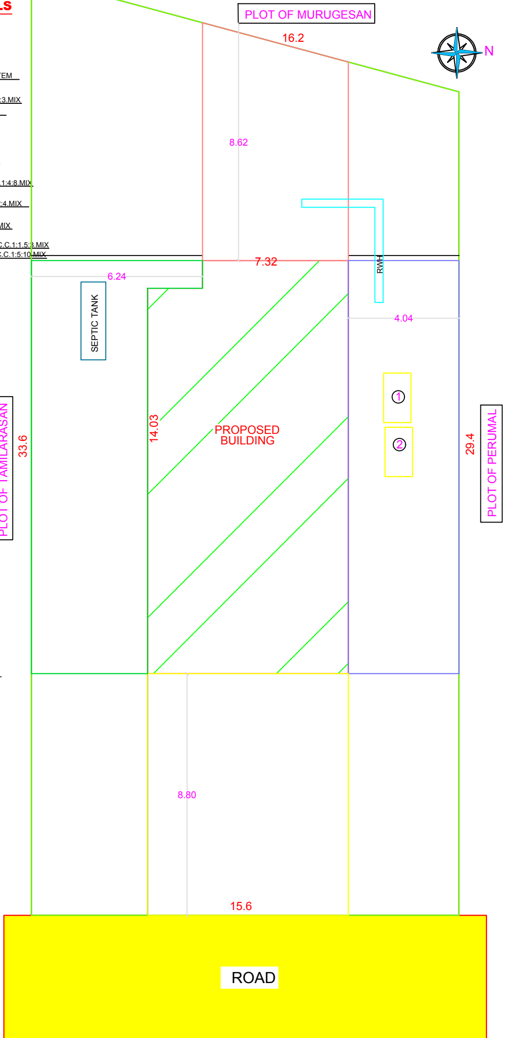
SITE PLAN
