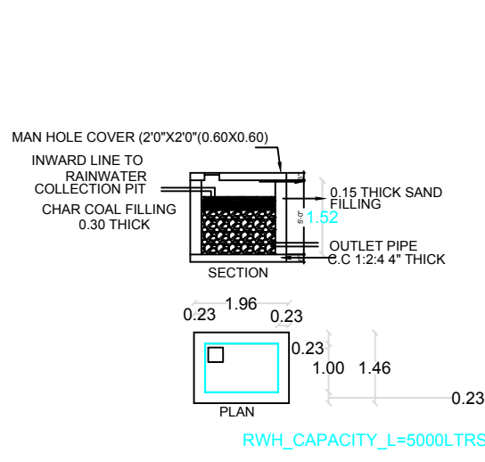
DETAILS OF RAINWATER HARVESTING
