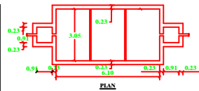
PLAN & SECTION OF SEPTIC TANK & DISPERSION TRENCH
