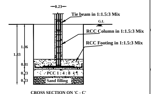
COLOUMN FOUNDATION DETAILS
