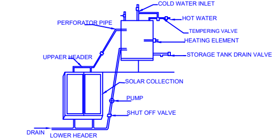
DETAILS OF SOLAR WATER HARVESTING (NTS)
