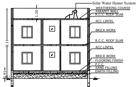
SECTION ON XX
