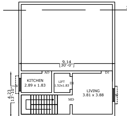
PRO. SECOND FLOOR PLAN
