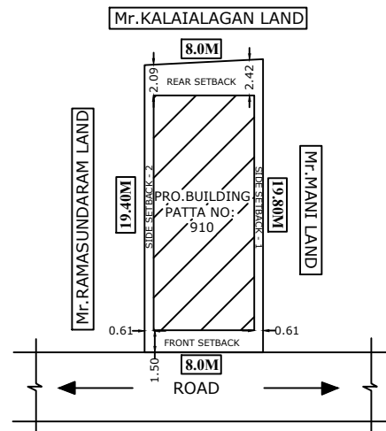
SITE PLAN
