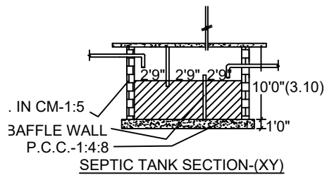
SEPTIC TANK SECTION-(XY)
