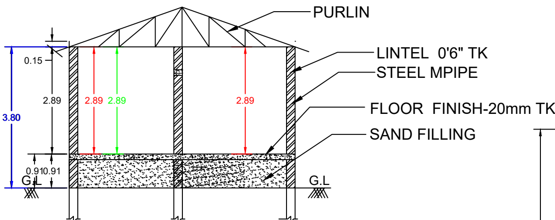
CROSS SECTION (A-B)
