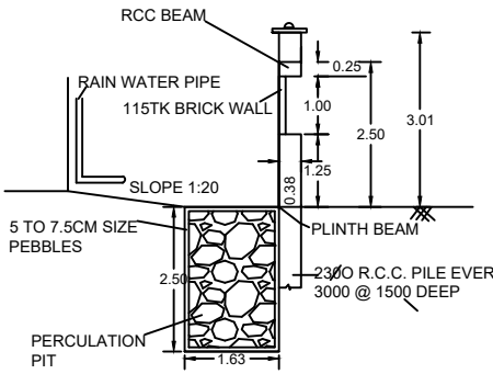
RAINWATER HARVESTING
