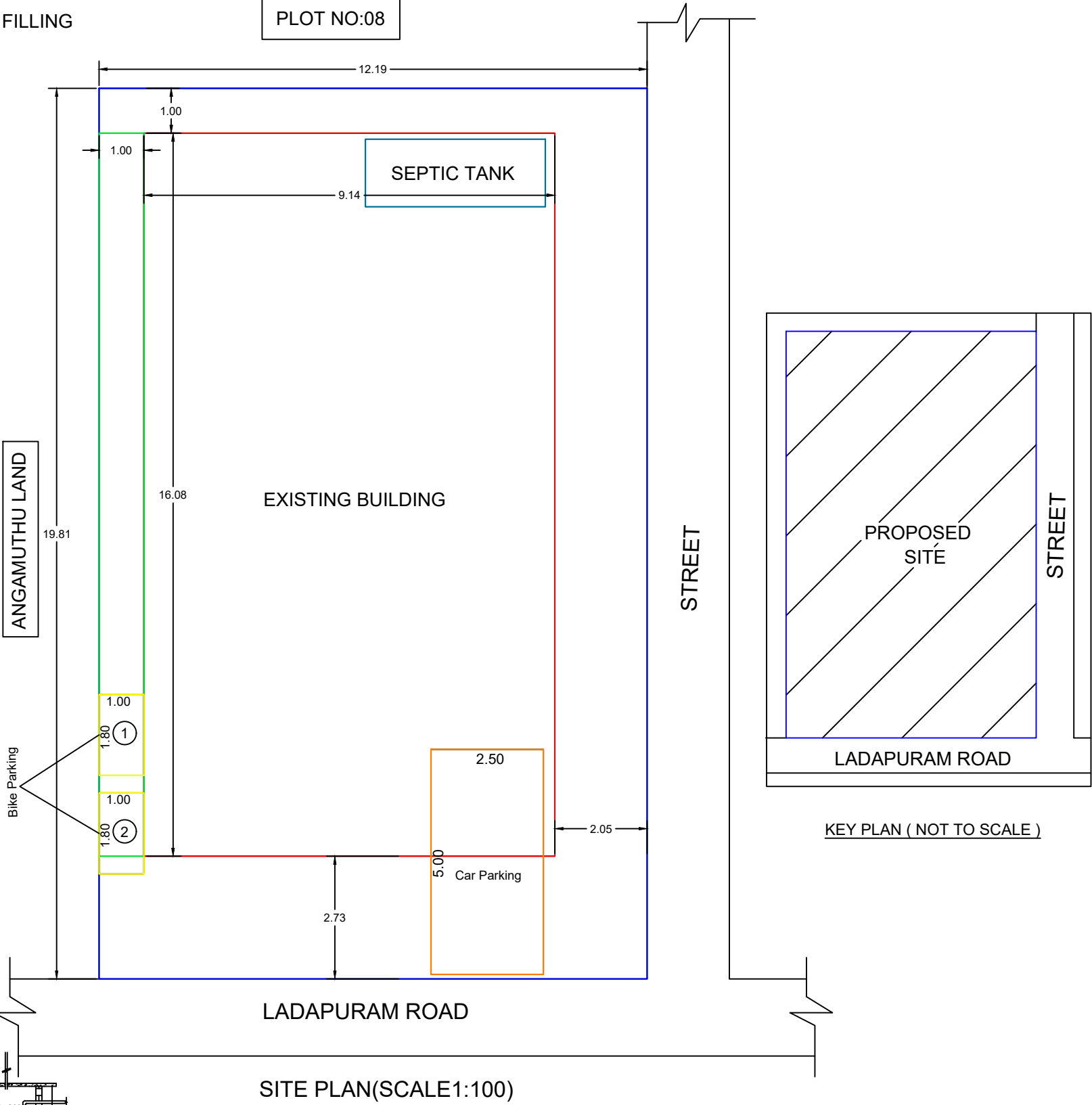
SITE PLAN(SCALE1:100)
