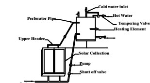
Details Of Solar Water Heater (NTS)
