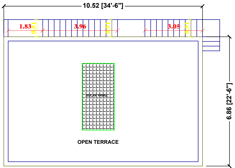
TERRACE PLAN
