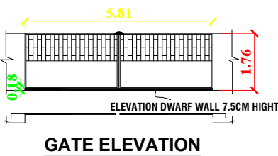
GATE ELEVATION
