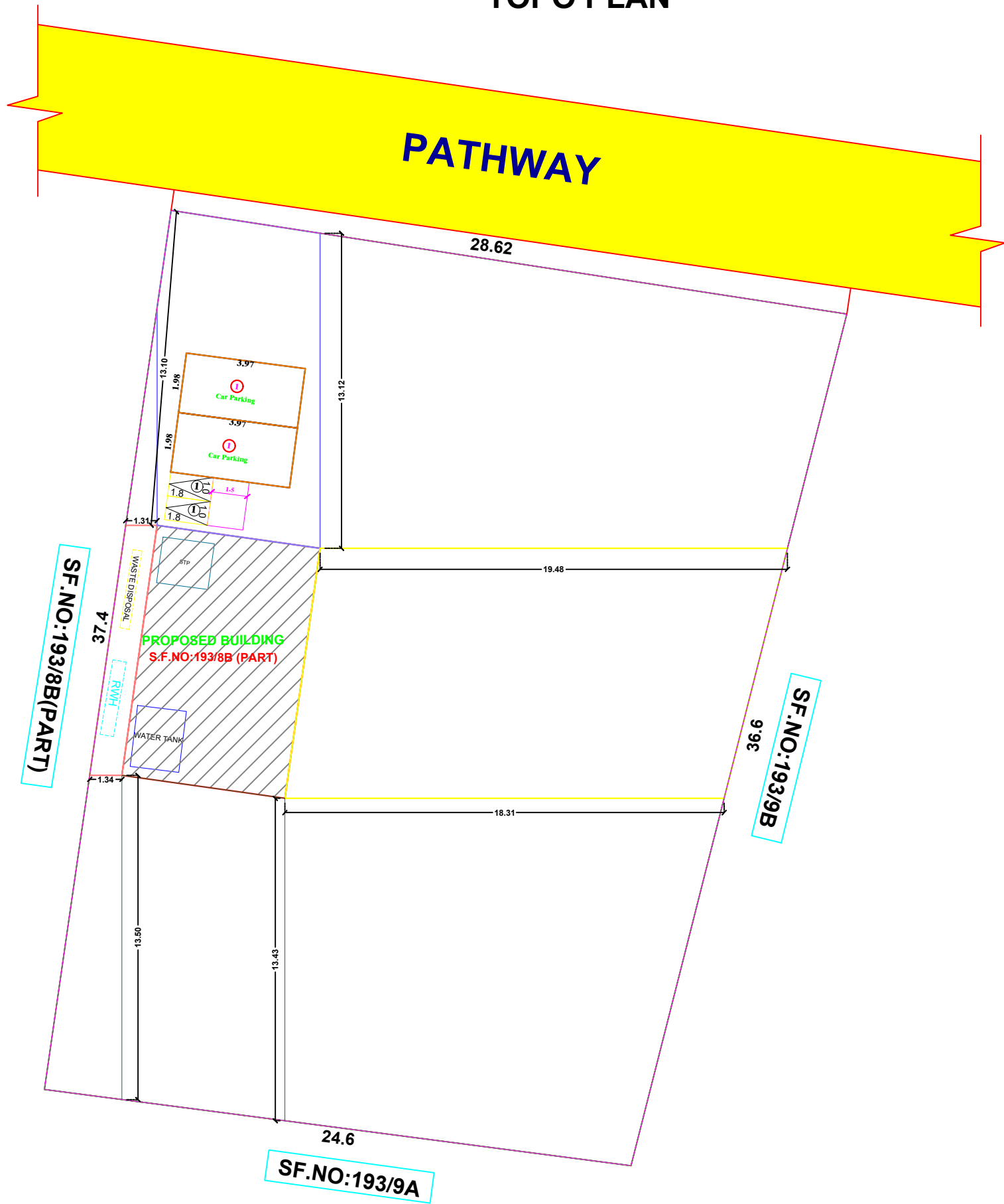
TOPO PLAN
