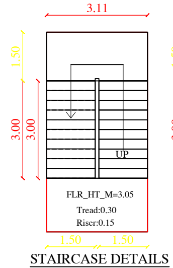
STAIRCASE DETAILS
