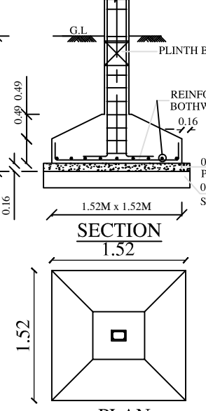
FOUNDATION DETAILS
