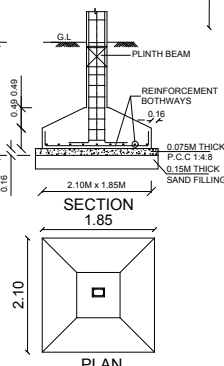
FOUNDATION DETAILS
