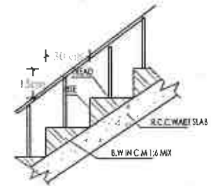
SECTION OF STAIRCASE
